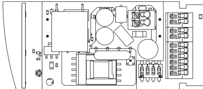
ORIONMETER LA-IP-RSP/AC
